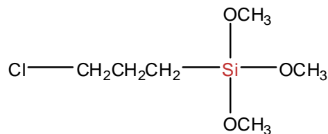
3-trimethoxysilyl-1-chloropropane
